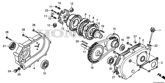
REDUCTION(2)
