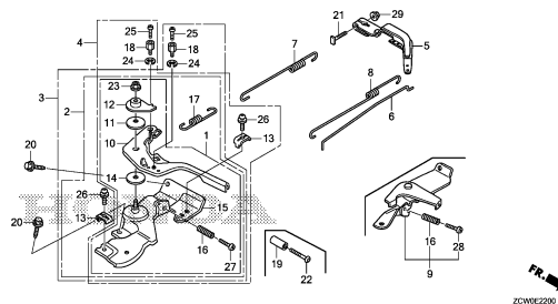
REDUCTION(2)
