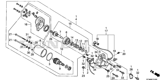
REDUCTION(1)
