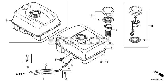
FUEL TANK
