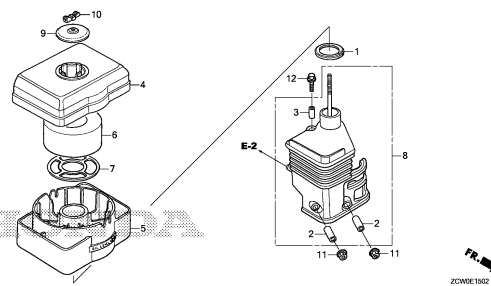
AIR CLEANER(OIL BATH)
